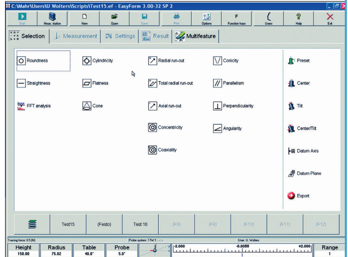
EasyForm 3.0
